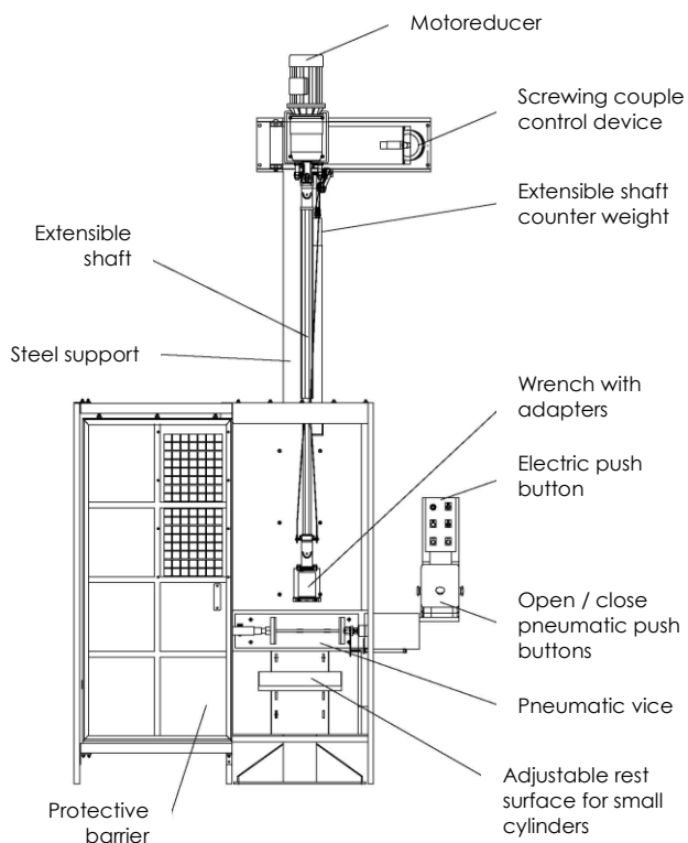
Complete equipment
